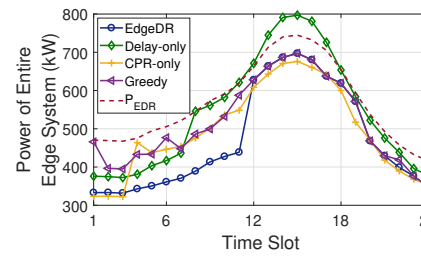
Fig. 9. Comparison of the entire edge system power within the edge demand response event with different mechanisms.
